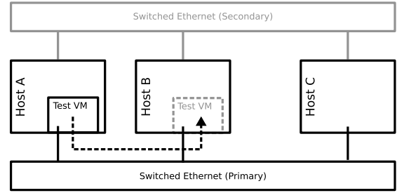
Figure 4. Experimental setup
